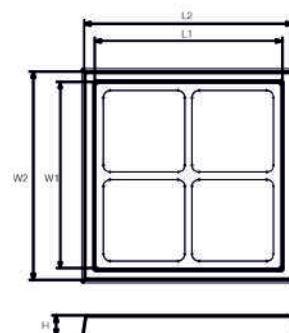
L1 - Inner Length, W1 - Inner Width, H - Height L2 - Outer Length, W2 - Outer Width
